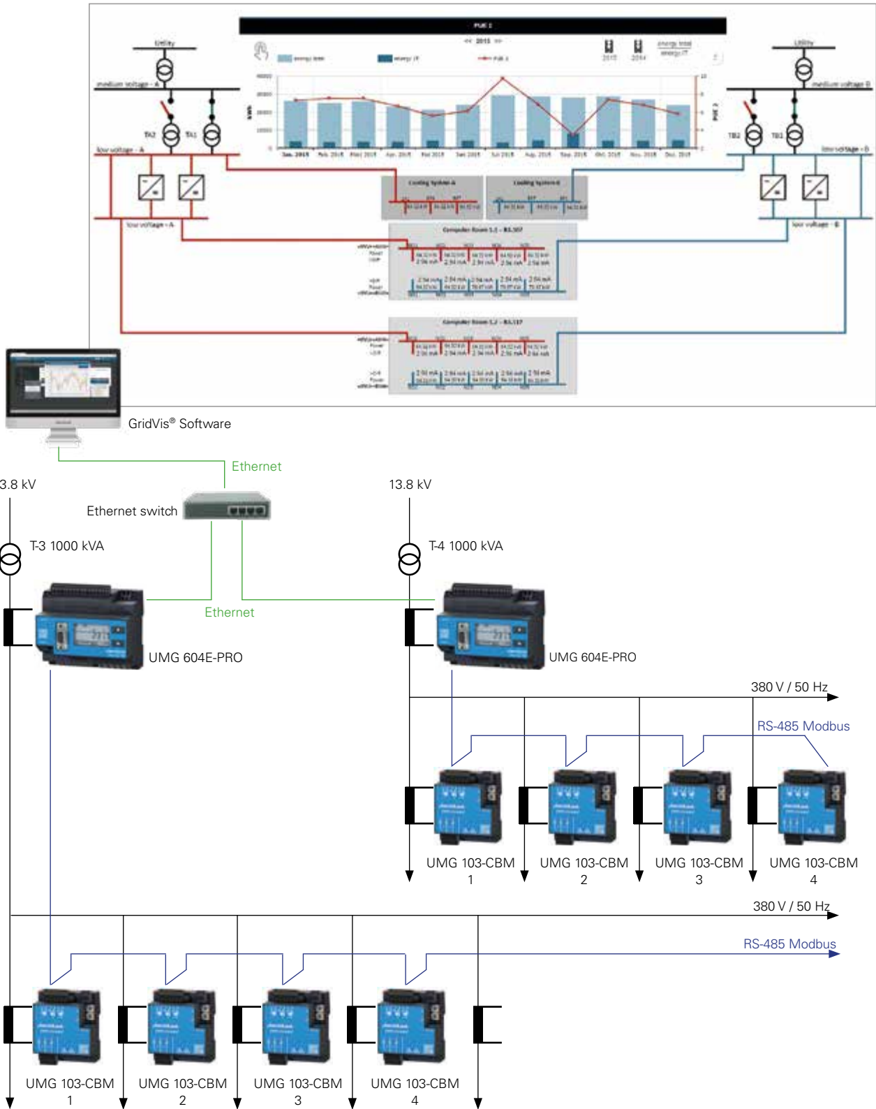
Fig.: Illustration of typical application with 2 feeders, UMG 604-PRO as master meters in the main feeder and UMG 103-CBM for measuring the low voltage outgoing feeders.
