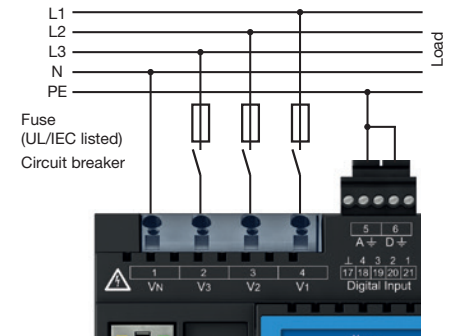
Fig. "Voltage measurement" connection example.
