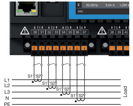
Fig. "Current measurement" connection example.
